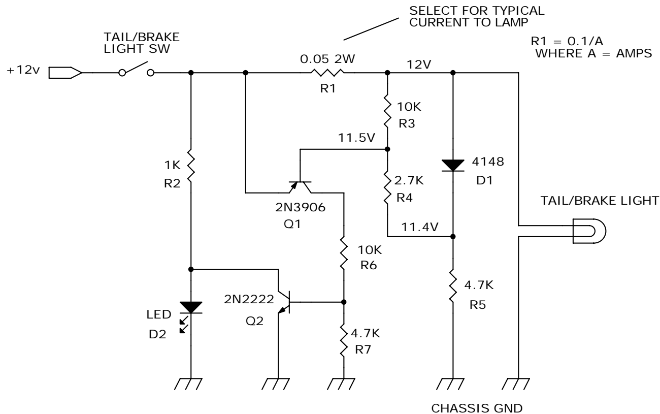
BAD BULB INDICATOR 4 AMP DETECTION WITH VALUES SHOWN
